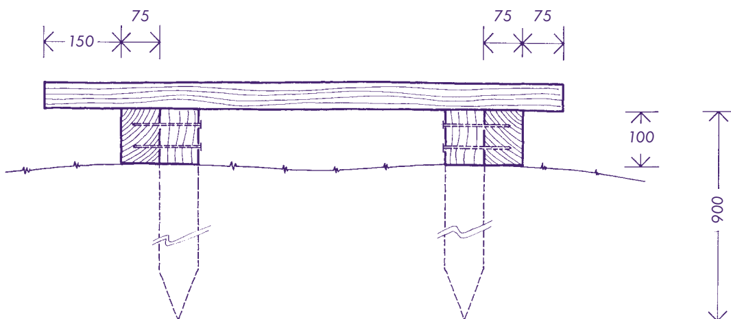
6.1B Section X-Y Scale 1:10 0 500mm
